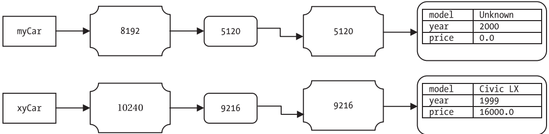
Figure 8-17. Memory state of reference variables myCar and xyCar and two Car objects
