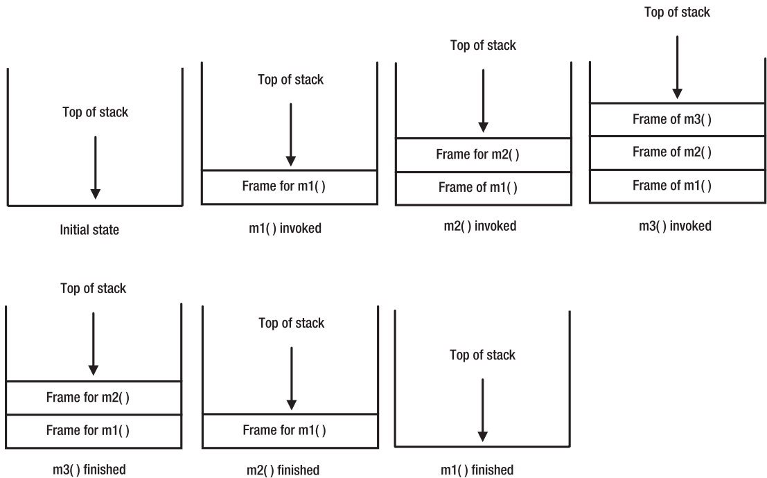
Figure 13-5. State of the stack of a thread when methods m1() , m2() , and m3() are called
