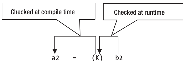
Figure 20-2. Runtime and compile-time checks made for downcasting
