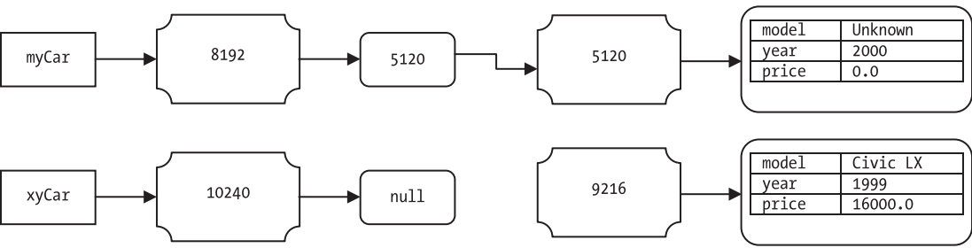
Figure 8-18. Memory state of reference variables myCar and xyCar and two Car objects after xyCar has been assigned a null reference
