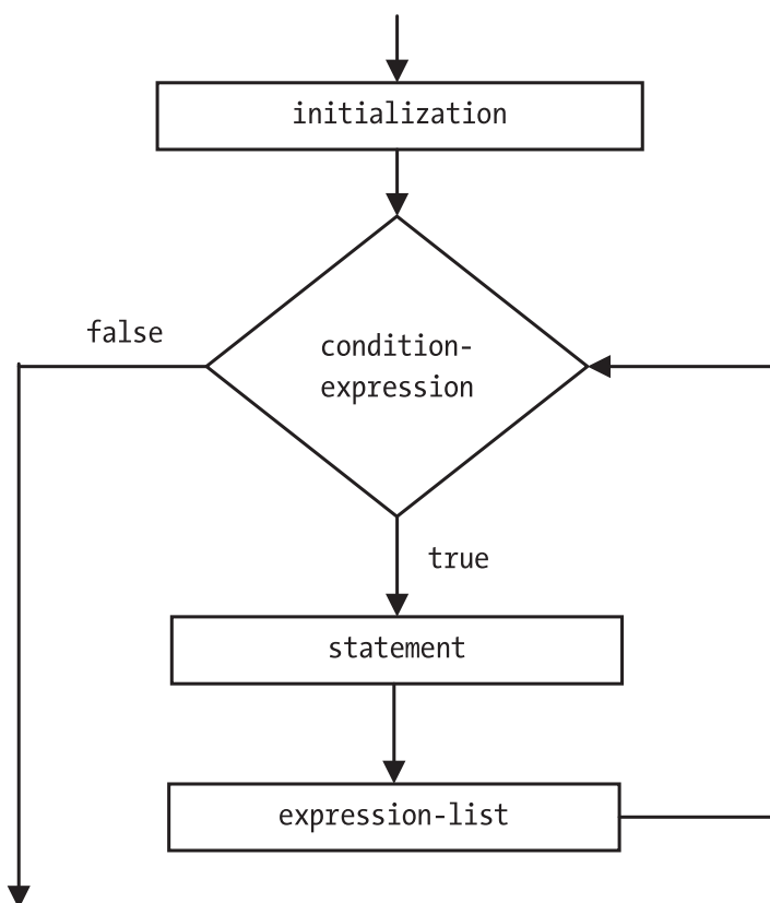
Figure 6-3. The flow diagram for a for-loop statement
