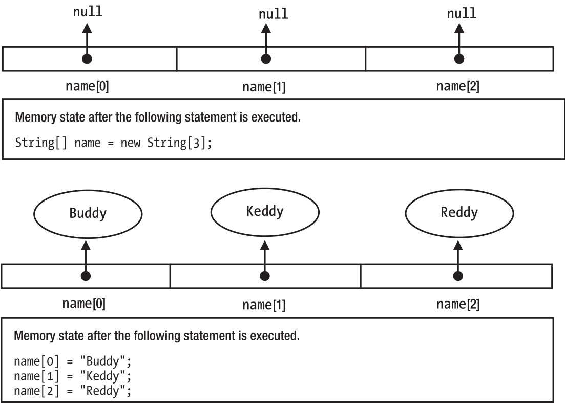
Figure 19-1. Reference-type array initialization
