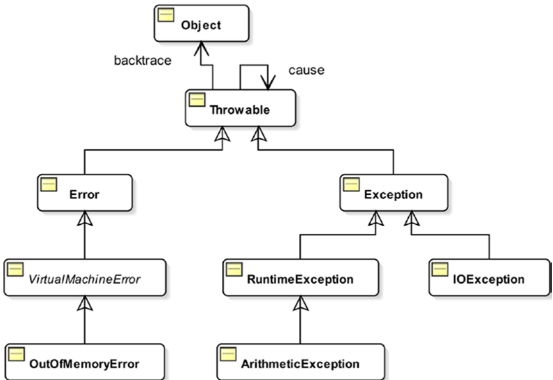
Figure 13-2. A few classes in the exception class hierarchy
