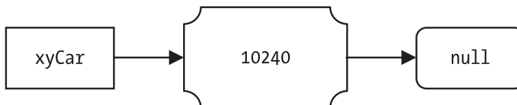
Figure 8-14. Memory state of xyCar reference variable
