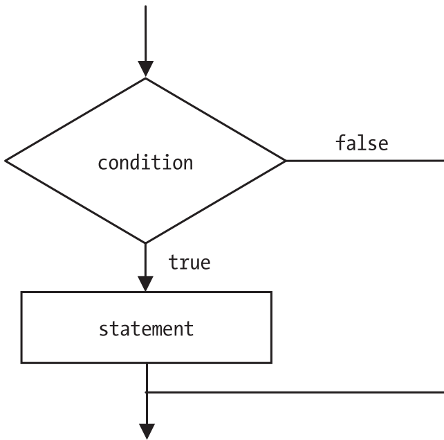
Figure 6-2. The flow diagram for an if statement
