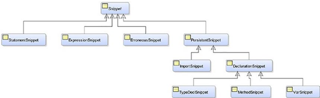
Figure 23-6. A class diagram for the Snippet class and its descendants
