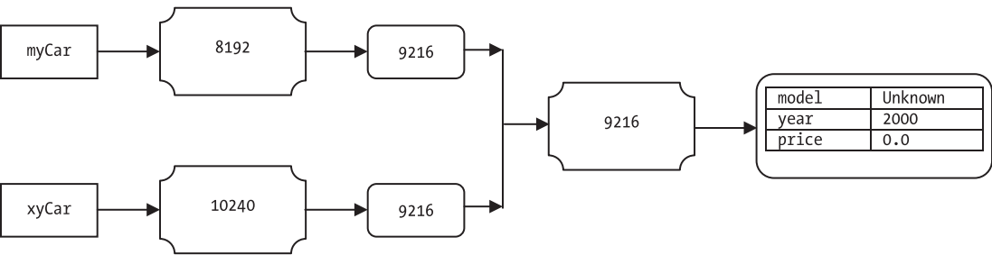
Figure 8-15. Memory state showing myCar and xyCar referencing the same Car object in memory
