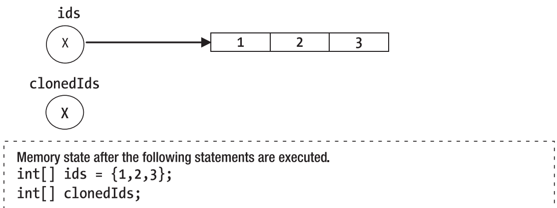
Figure 19-2. The ids array is populated, and the clonedIds array is declared
