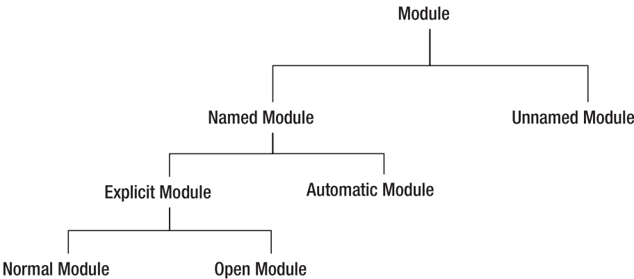
Figure 10-8. Types of modules
