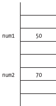
Figure 4-2. Memory state after two int type variables are assigned a value
