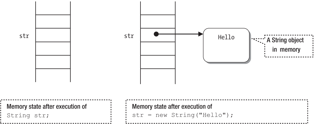
Figure 4-4. Memory states using reference variables
