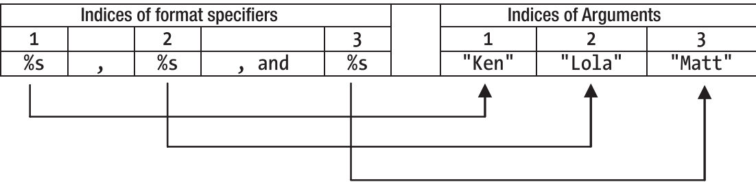
Figure 17-1. Indexes of format specifiers in a format string and indexes of the arguments
