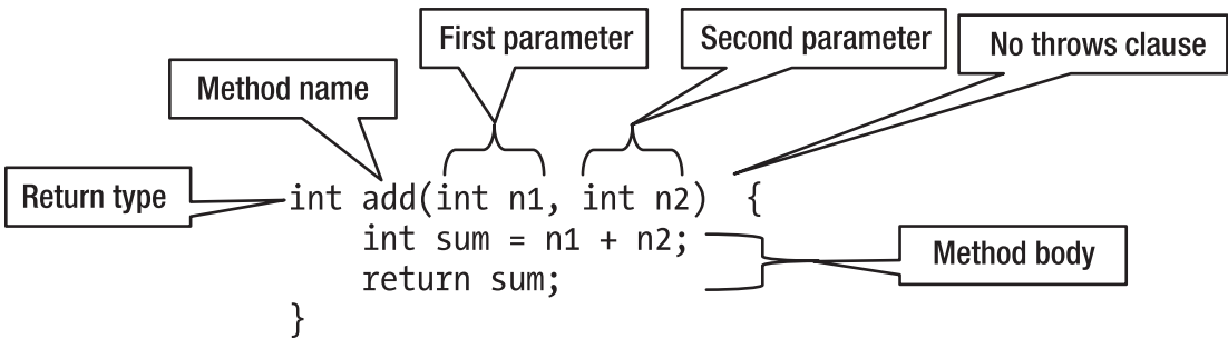
Figure 8-1. Parts of the add method
