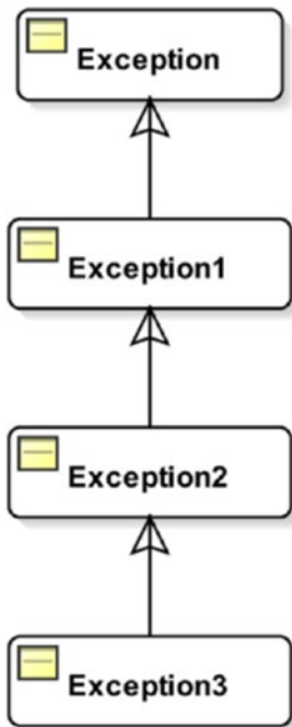
Figure 13-3. The class hierarchy for Exception1 , Exception2 , and Exception3 exception classes
