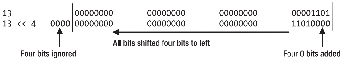
Figure 5-1. Computing 13 \ll 4
