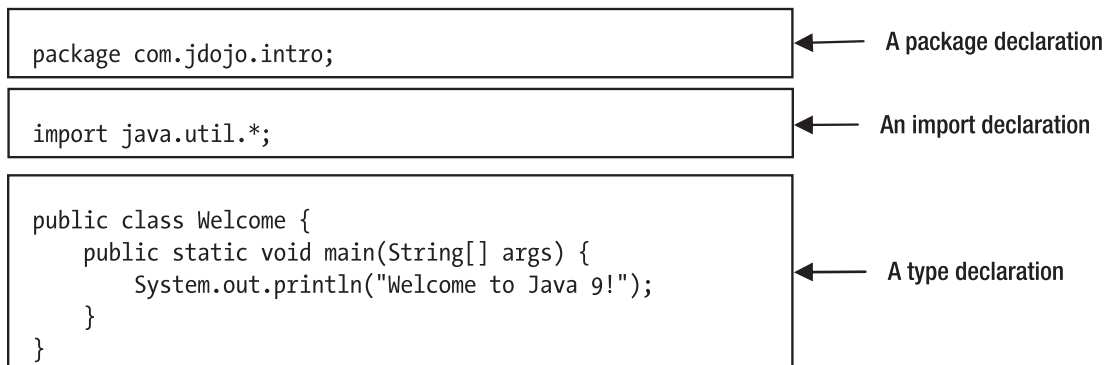
Figure 3-2. Parts of a compilation unit
