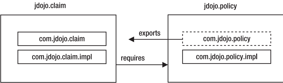
Figure 10-1. Declaring dependency between modules
