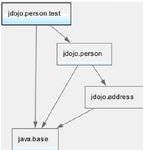
Figure 10-4. The module graph of the jdojo.person.test module
