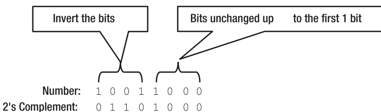
Figure 4-8. Computing 2's complement of a binary number
