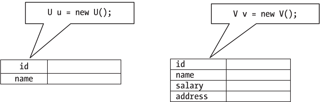
Figure 20-3. Memory allocation for an object includes all instance variable of the class and all its ancestors
