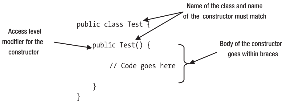
Figure 9-1. Anatomy of the constructor for the Test class
