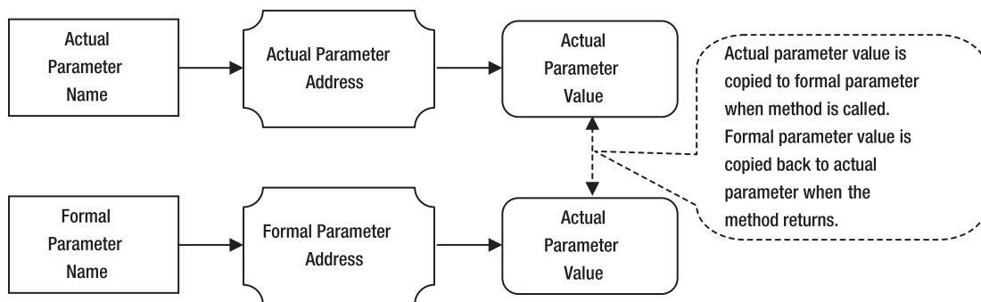
Figure 8-8. Memory states for actual and formal parameters when the pass by result parameter-passing mechanism is used
