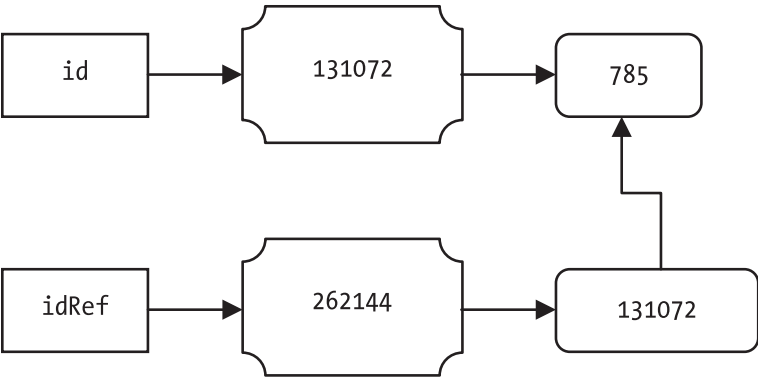
Figure 8-3. Difference between a variable and a reference variable
