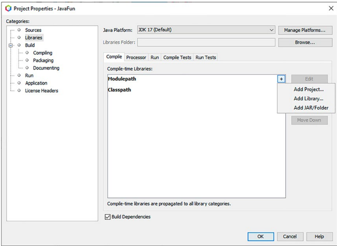
Figure 10-3. Setting the module path for a project in NetBeans
