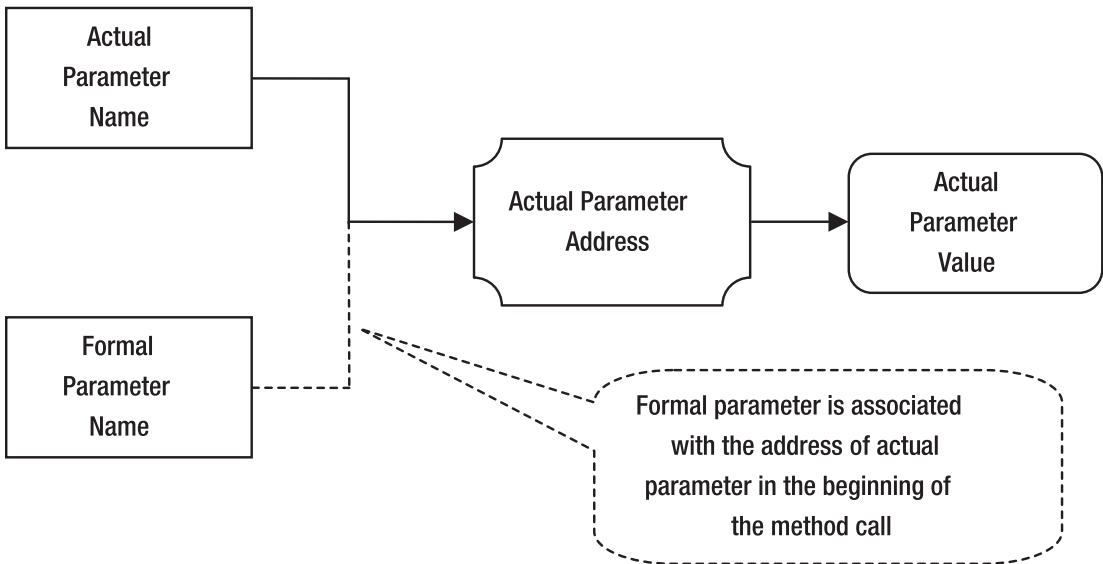
Figure 8-5. Memory states of actual and formal parameters when the parameters are passed by reference
