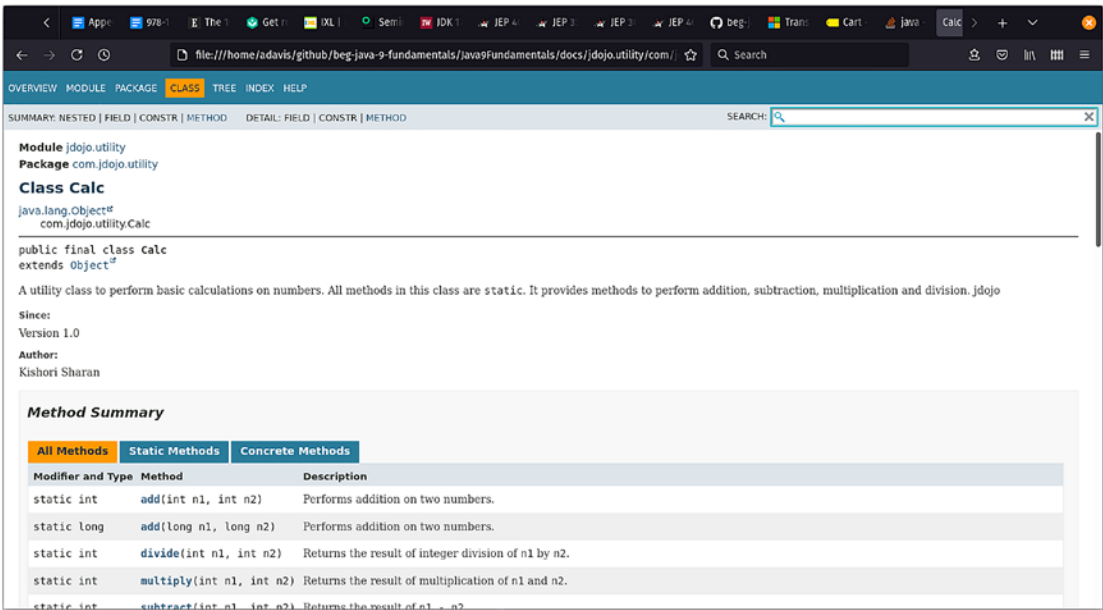
Figure B-2. The generated HTML page for the Calc class
