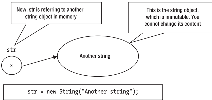
Figure 15-2. Assigning a different String object reference to a string variable
