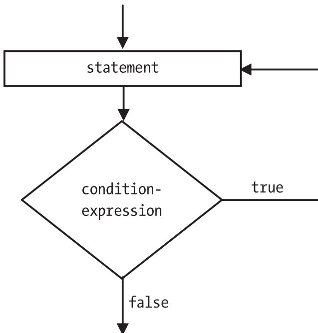
Figure 6-5. The flow diagram for a do-while statement
