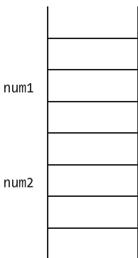
Figure 4-1. Memory state when two int type variables are declared
