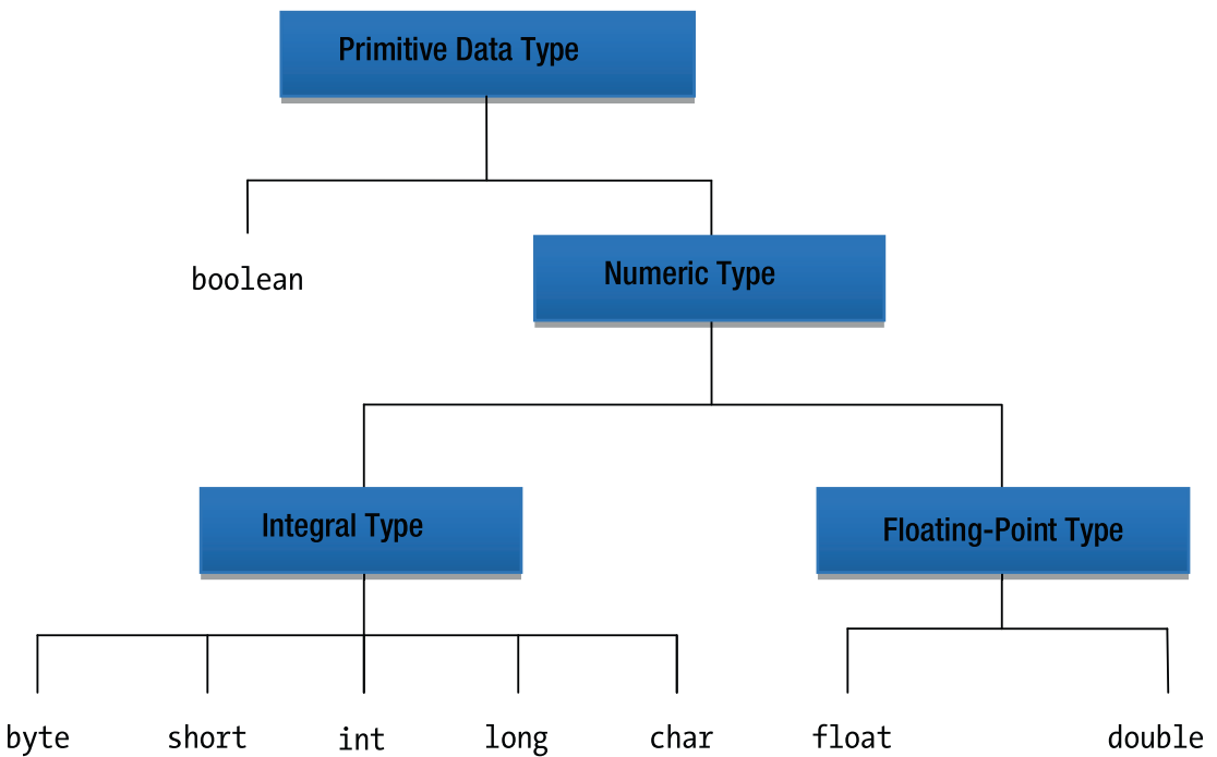
Figure 4-6. List of primitive data types divided by their categories in Java
